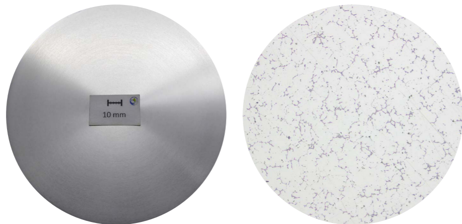
Macrosection, d178 mm: Segregation 2 mm Microsection, d178 mm (25 times magnification)
